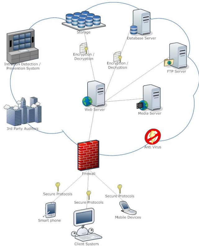
Figure 1. High Level Cloud Storage Architecture.
